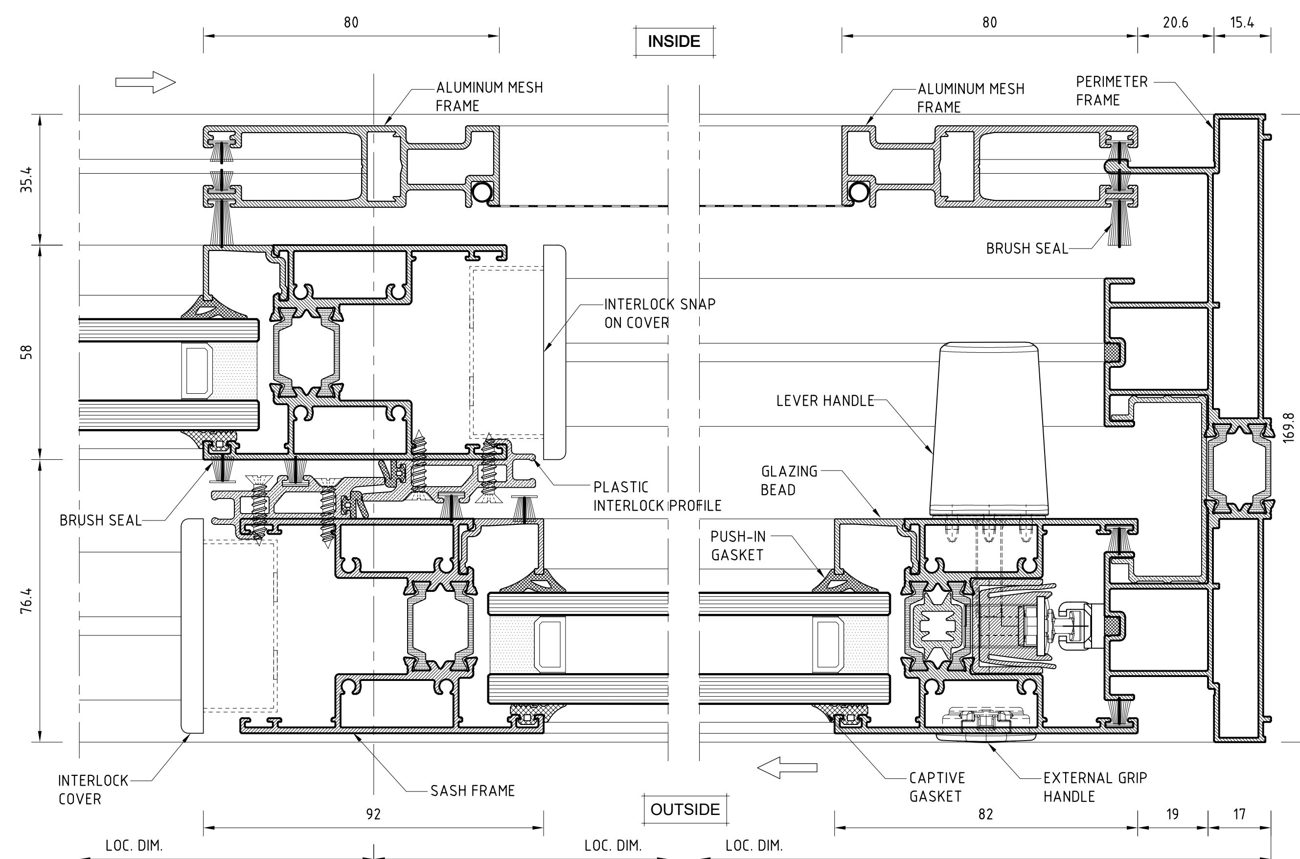
INTERLOCK DETAIL
